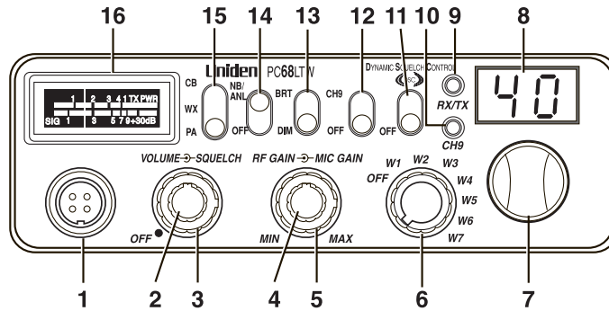
FRONT VIEW PC681TW BACKLIGHED PANEL
